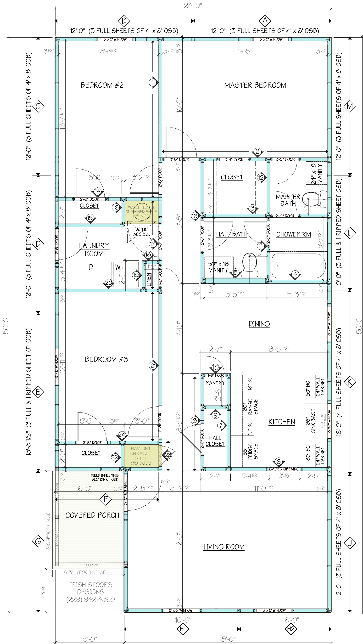
FLOOR PLAN & WALL PANEL LEGEND PLAN 303-KR (KITCHEN RIGHT) SCALE: 1/4" = 1'-0" DATE: 28-APR-2007
